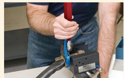
Handle-less strap wrench, digital torque wrench, strain relief, backshell (in vise jaws), connector, vise
