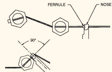
FIGURE 16: Position of Safe-T-Cable® Tool
