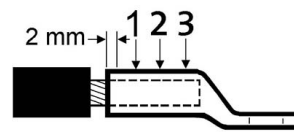
Crimp sequence for three crimps.
