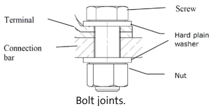
Bolt joints.
