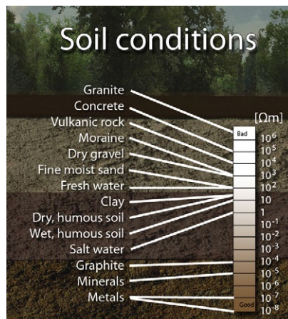
1. Resistivity in different soil conditions.
