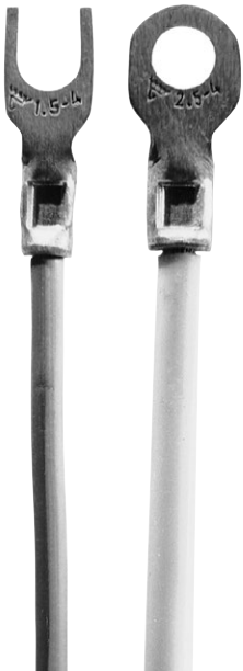
Examples of crimps using Elpress uninsulated terminals.
