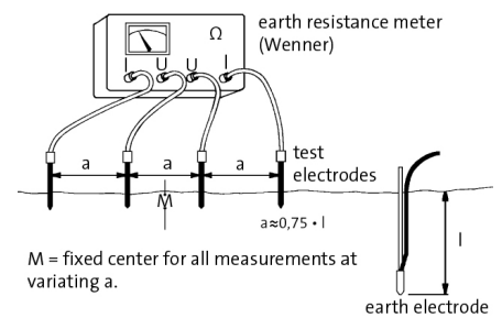
Measurement of ground resistance.
