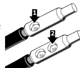
Crimp sequence
